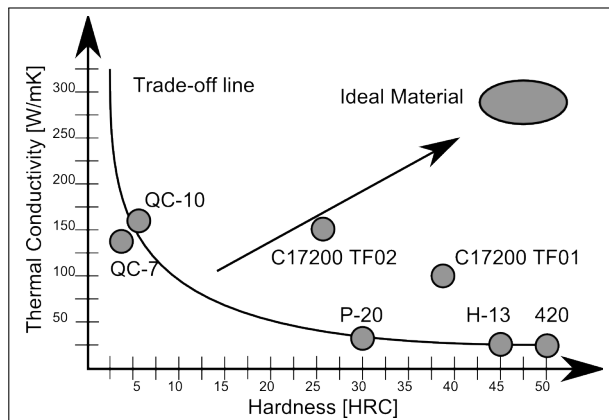
Figure 2: The ideal material for mold cores and cavities is one that has both excellent thermal conductivity and high hardness (note: the aluminum alloys have hardnesses below the effective range of the HRC scale)
